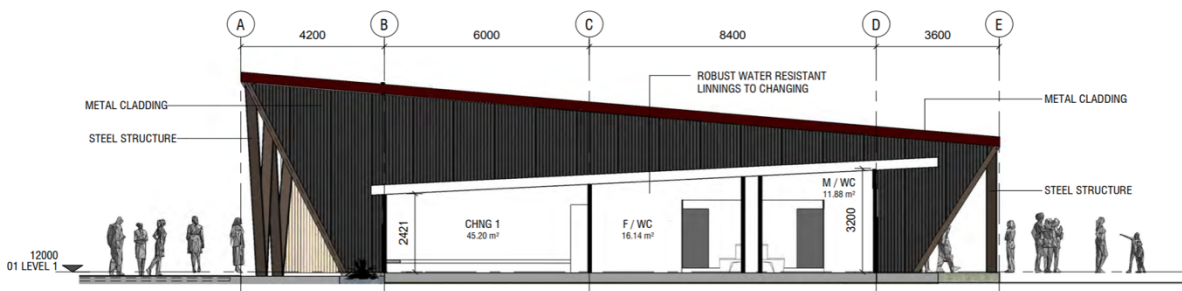
1 Section 02 CHANGING SHEDS 1:100
