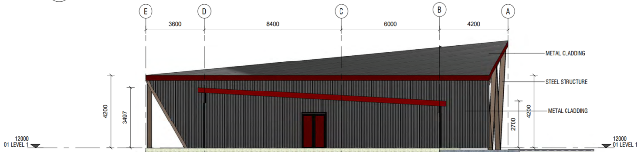
2 WEST ELEVATION CA-100 1:100
