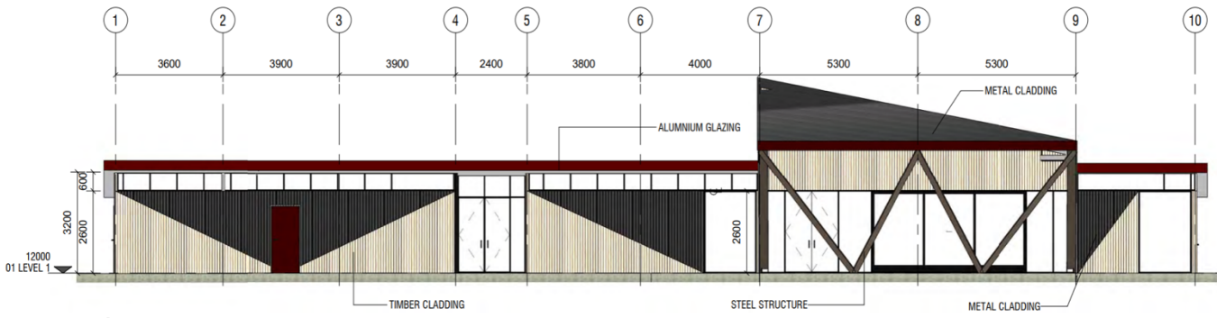
1 SOUTH ELEVATION CA-100 1:100
