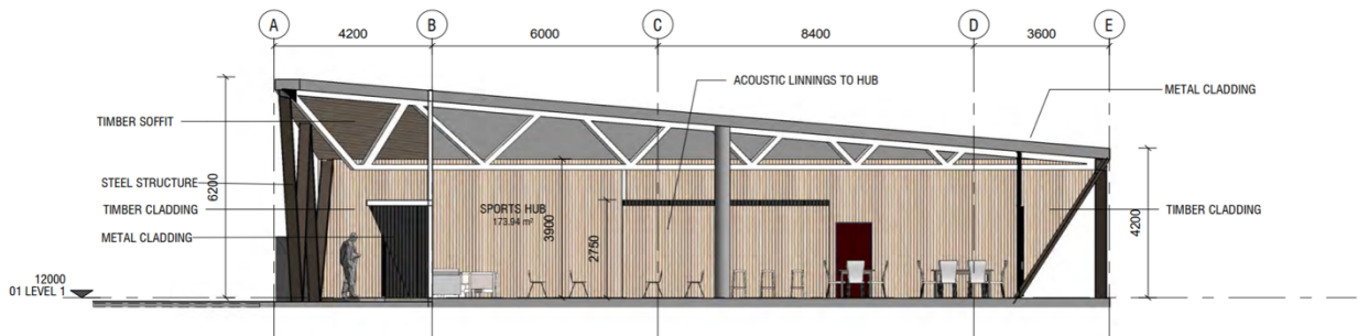
2 Section 01 - SPORTS HUB 1:100
